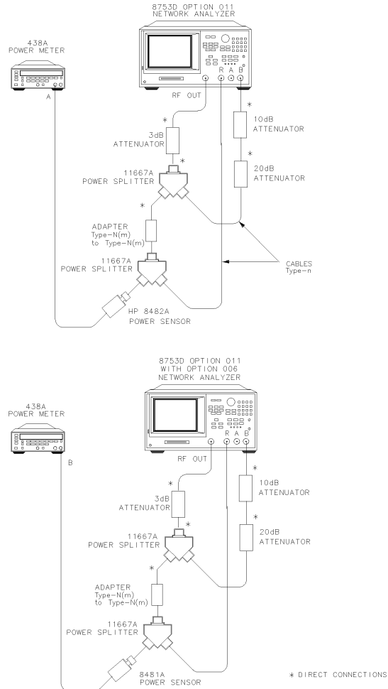
Figure 6-31. Channel R Phase Compression Test Setup
