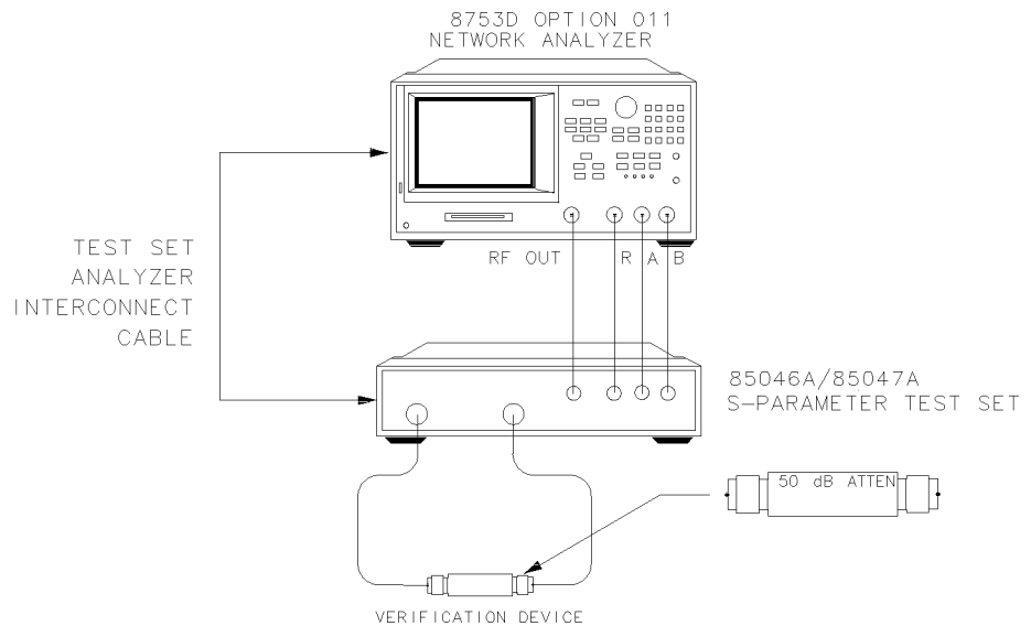
Figure 5-5. Connections for the 50 dB Verification Device
