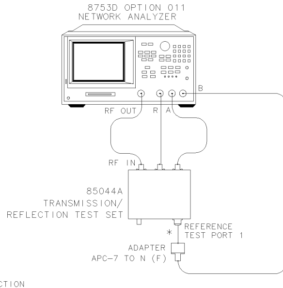
Figure 5-10. Transmission Calibration Setup
