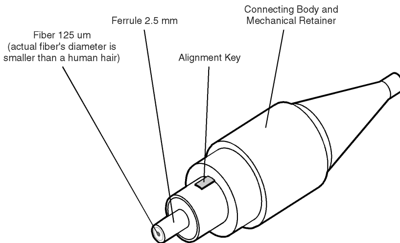
Figure 1 Basic components of a connector.
