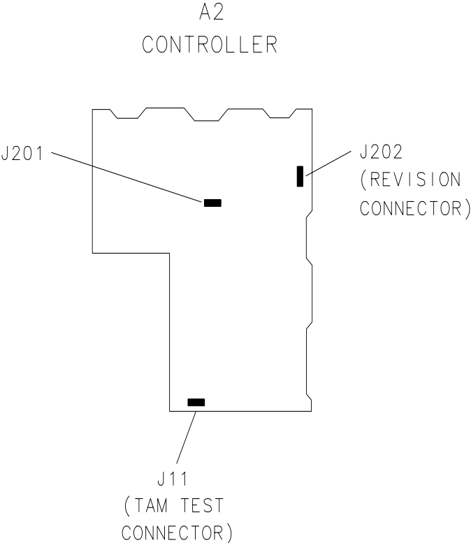
Figure 10-1 A2 Test Connectors
