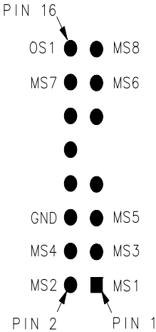
Figure 10-2 A2 Test Connector Pin Locations
