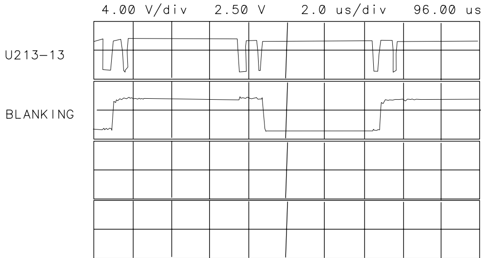
Figure 10-5 Expanded Blanking Waveforms
