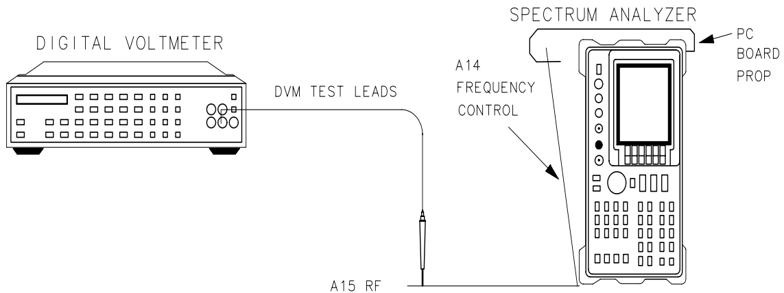
Figure 3-11 Sampler Adjustment Setup
