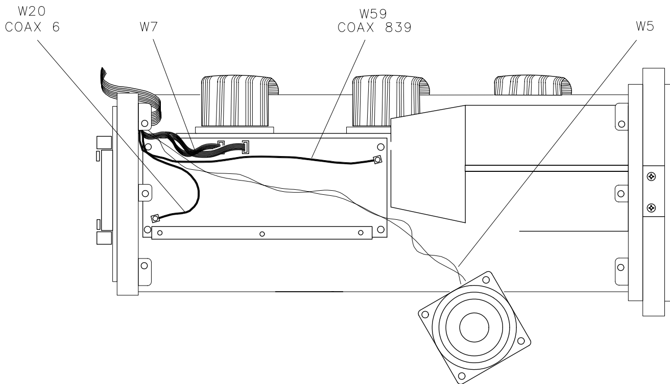
Figure 6-7 A16 Fast ADC (Option 007)
