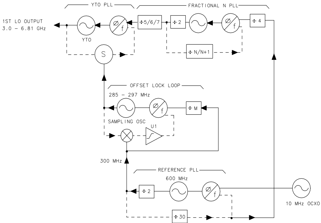
Figure 7-7 Phase Lock Loops
