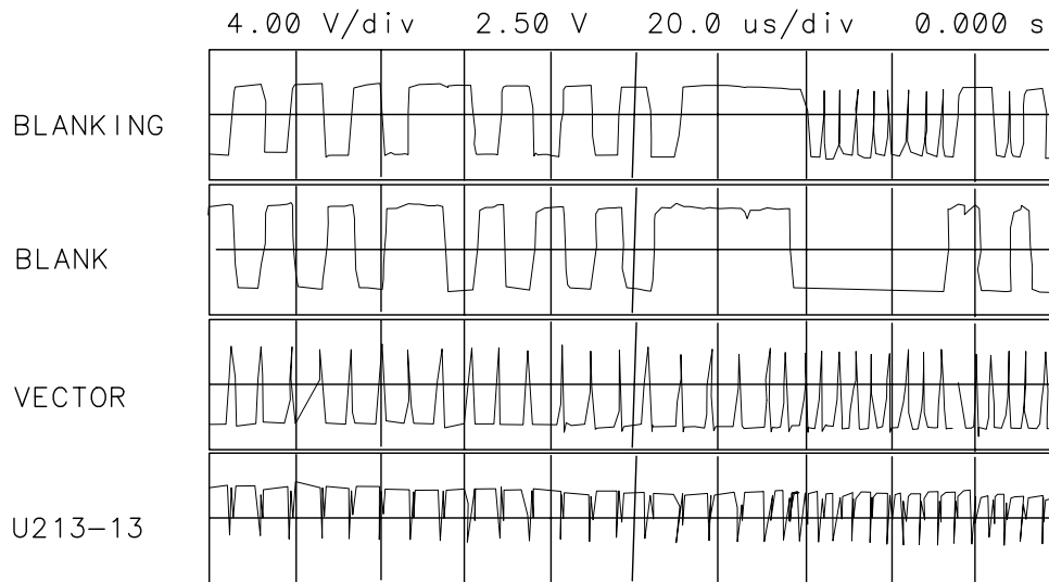
Figure 10-4 Blanking Waveforms
