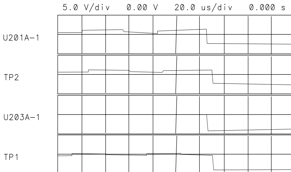
Figure 10-8 Expanded X/Y Line Generator Waveforms
