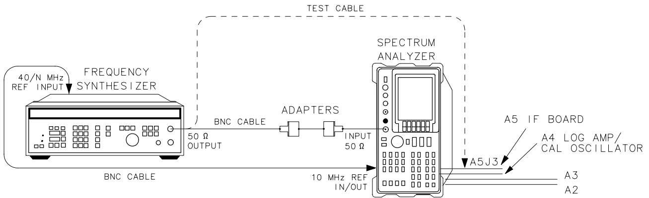
Figure 2-7 DC Log Adjustment Setup
