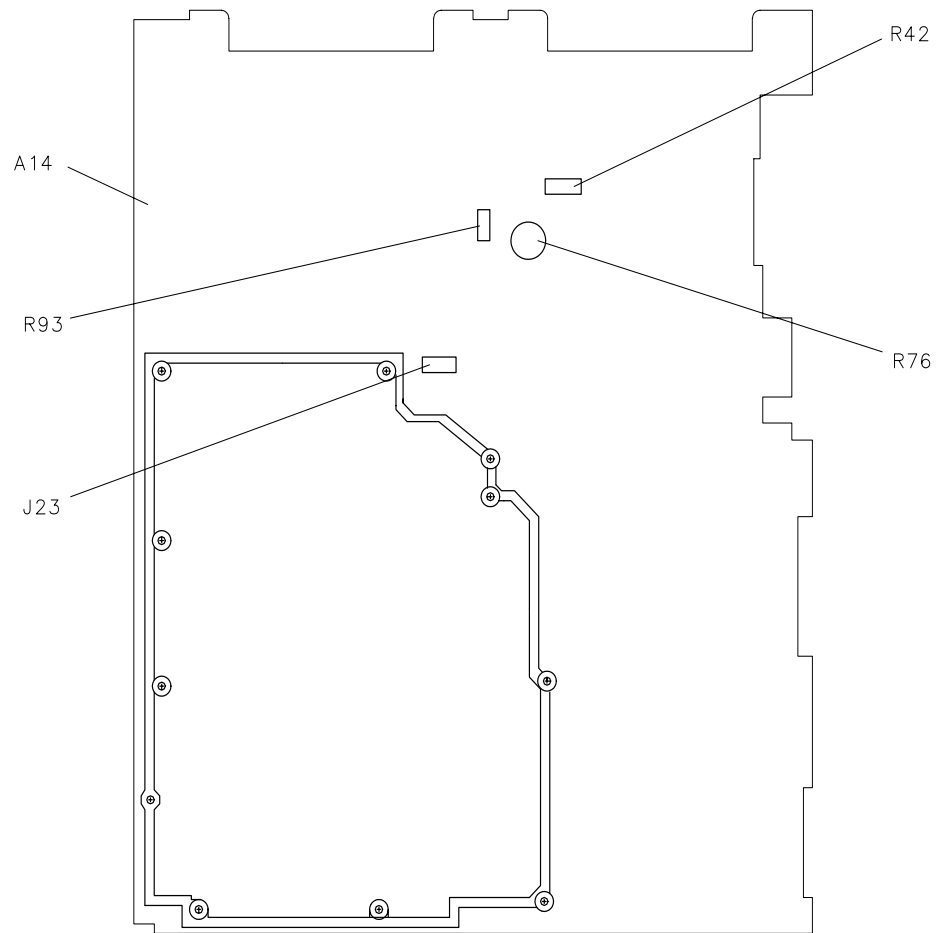
Figure 2-3 YTO FM Coil Adjustment Locations
