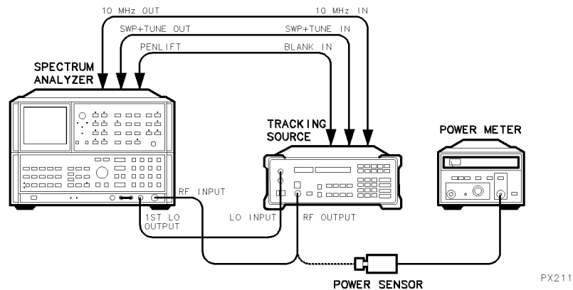
Figure 2-2. HP 85645A Maximum RF Power Level Setup
