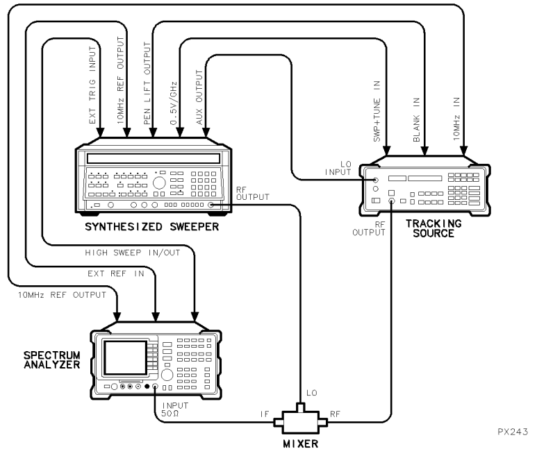
Figure 3-4. Connecting the Mixer to Measure Conversion Loss
