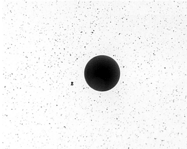
Figure 5-4. Clean, problem-free fiber end and ferrule.
