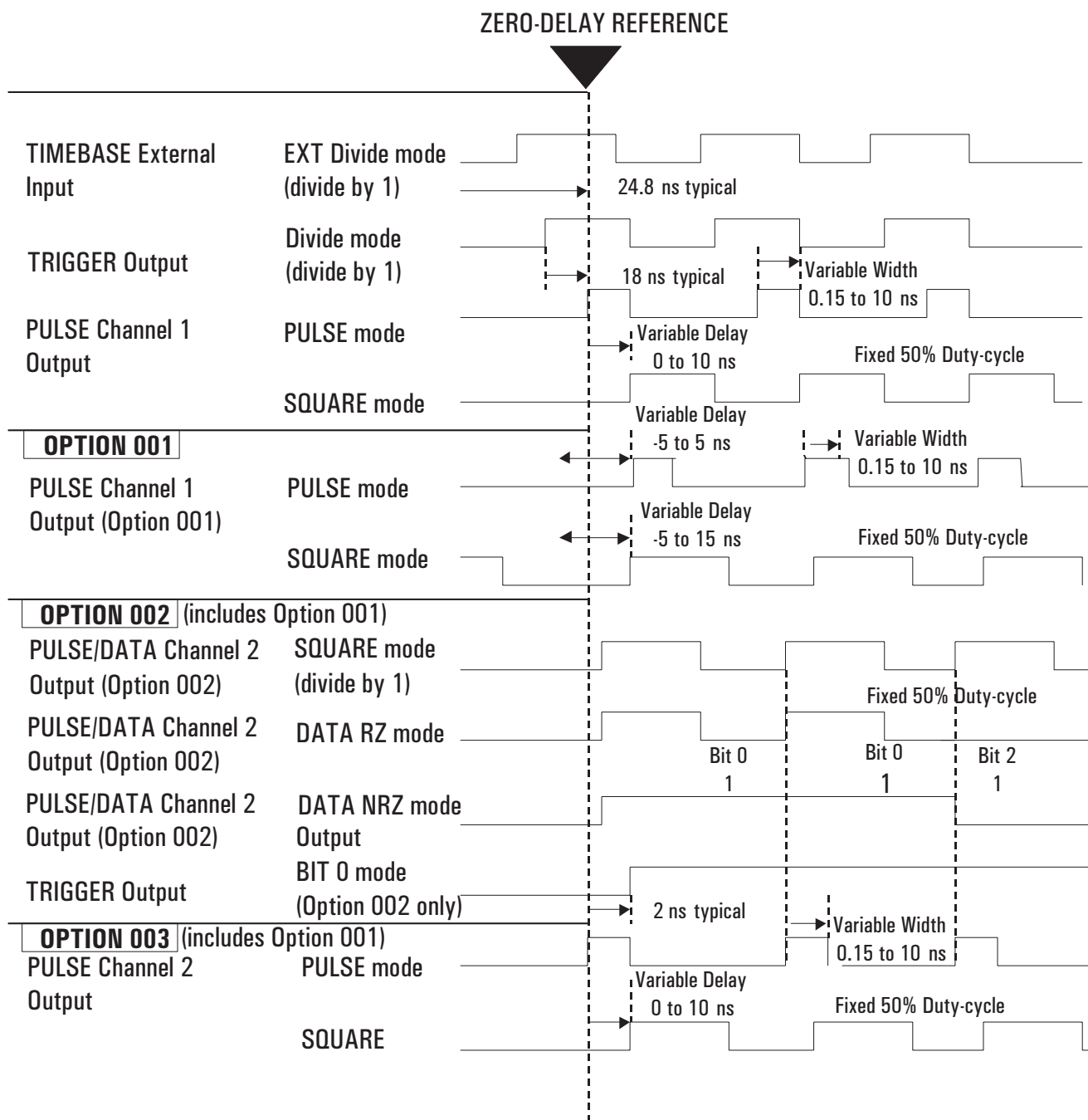
Interchannel Timing Diagram
