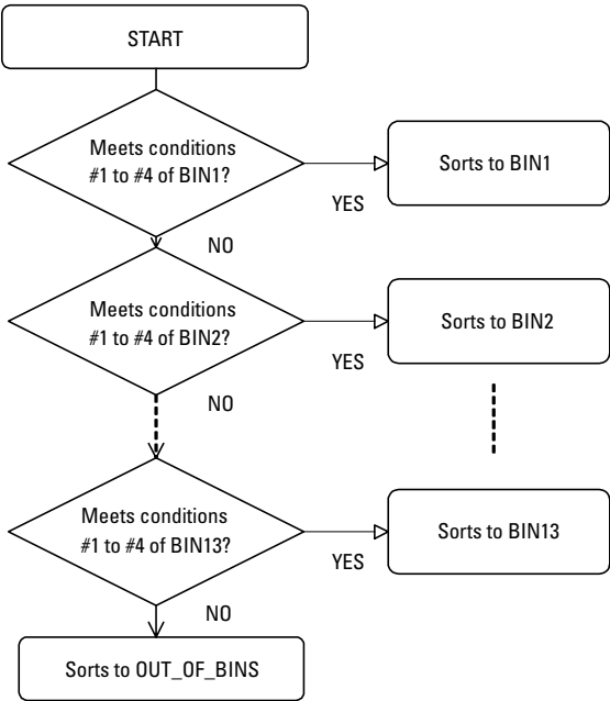
Figure 5. Bin-sort sequence
