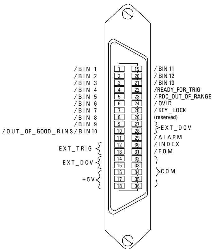
Figure 7. Pin location of handler interface
