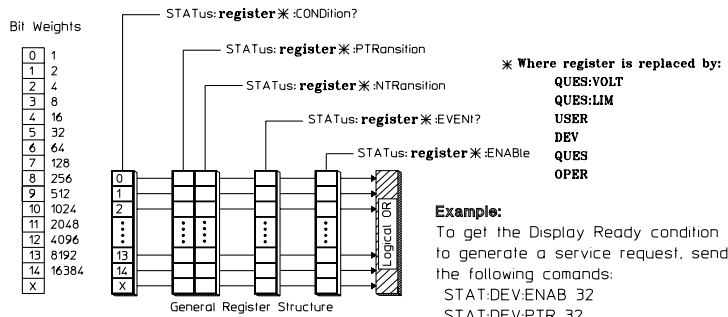
Figure 1. HP 35670A Status Register Summary
