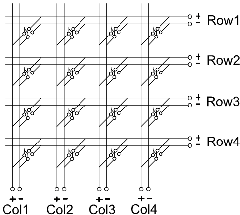
Matrix Switching
