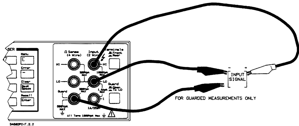
Figure 24. Digitizing measurement connections
