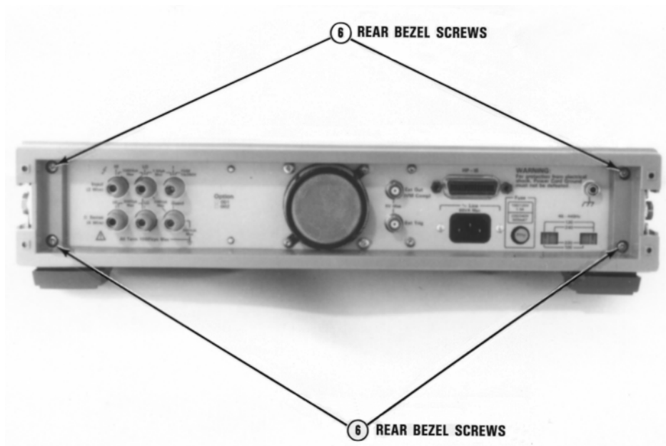
Figure 38. 3458 Rear view
