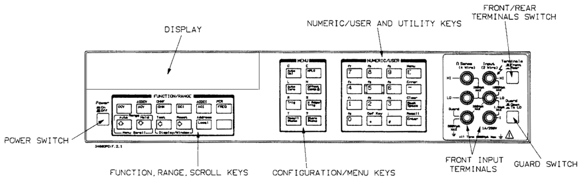
Figure 6. Front Panel
