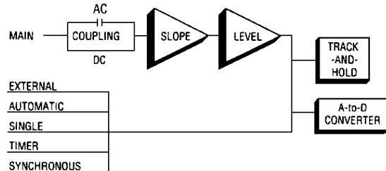
Figure 54. The trigger event choices shown provide the versatility needed to match a wide variety of applications.
