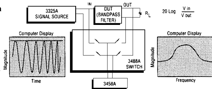
Figure 57. Using the 3458A as a phase/gain meter with a swept frequency generator for magnitude only Bode plots. The DUT can be characterized over frequency with a phase synchronous trigger to time the measurement.
