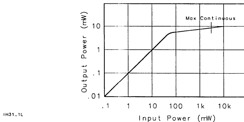
Figure 1-1. Typical Limiting Characteristics
