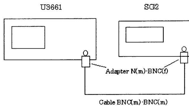
Figure 3-6 Setup of RBW Selectivity Test
