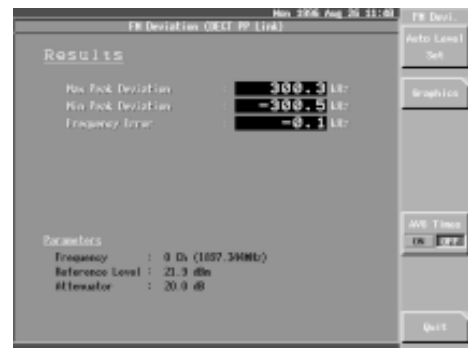
▲ DECT FM deviation measurement
