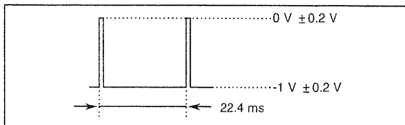
Figure 8-6 PATTERN TRIGGER Output Waveform (PRBS, N = 23 , f = 12000 \text{ MHz} , 5 \text{ ms/div} )
