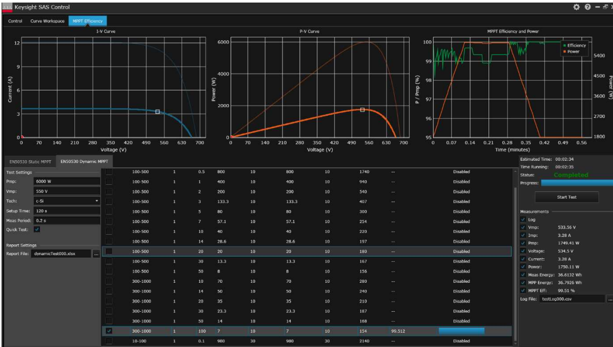
Figure 17. SAS Control Software performing dynamic EN50530 MPPT test
