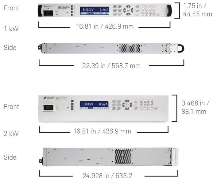
Figure 6. 1 kW and 2 kW power supplies, front and side dimensions.
