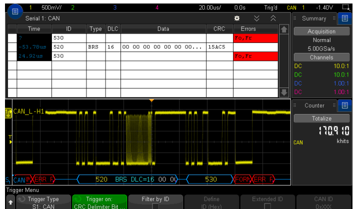
Figure 28. Totalizer counts the number of events. In addition, it can count the number of trigger-condition-qualified events as fast as 25 million events a second.
