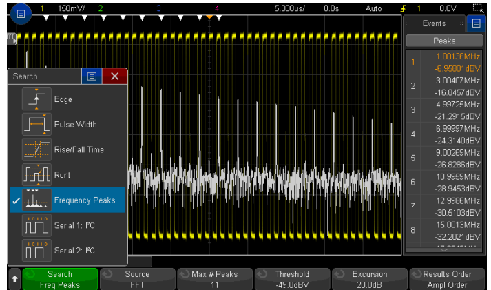
Figure 14. The 3000T X-Series was set up to capture clock signals for FFT analysis. Using the search and navigation capability, the scope was able to find, mark (white triangles) and quickly navigate to the first 11 frequency peak occurrences. You can sort it in the order of frequency or amplitude.
