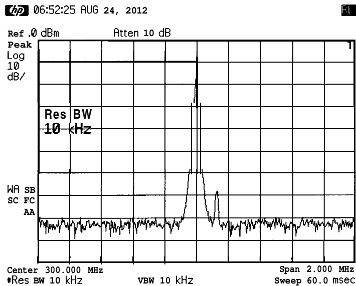
Figure 2-7 Signal Resolution with a 10 kHz Resolution Bandwidth
