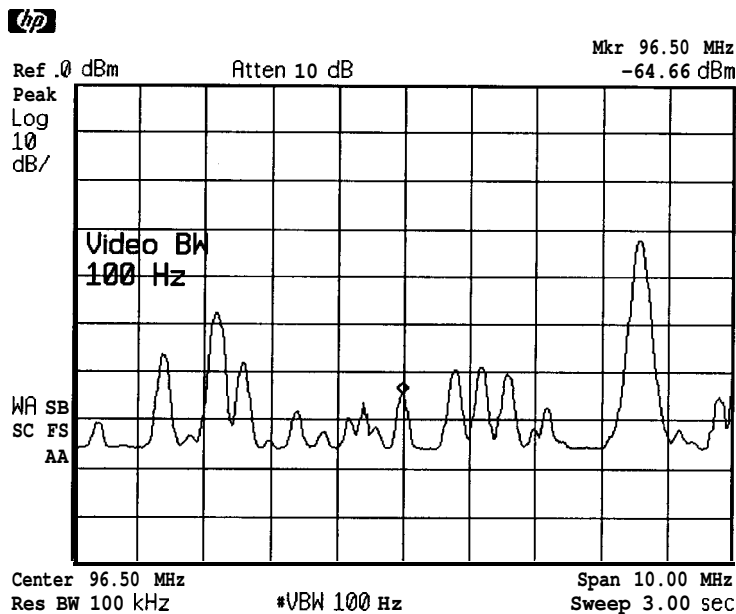
Figure 2-17 Decreasing Video Bandwidth
