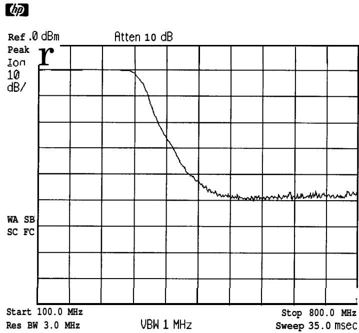
Figure 3-3 Spectrum Analyzer Settings According to the Measurement Requirement
