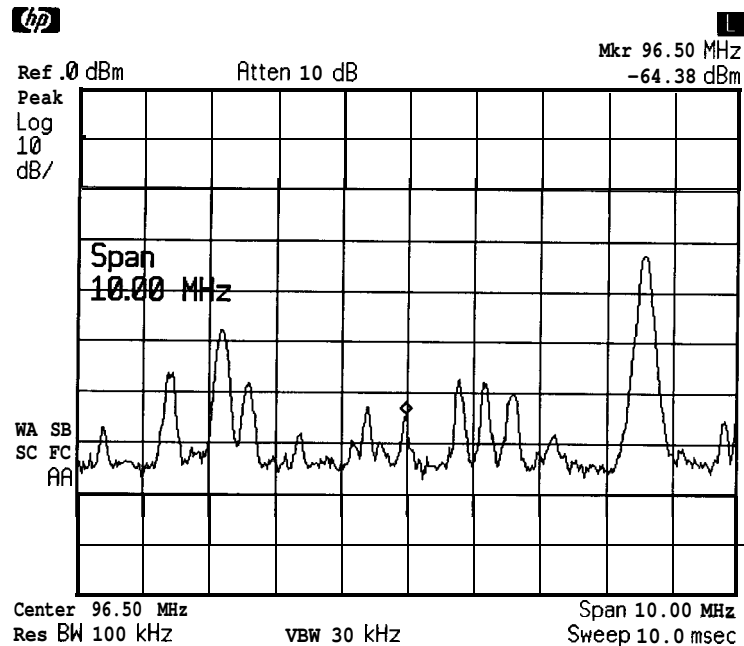
Figure 2-14 Low-Level Signal
