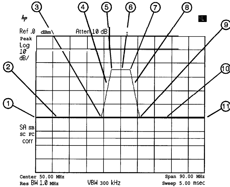
Figure 4-4 Limit Line Segments
