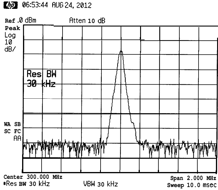
Figure 2-8 Signal Resolution with a 30 kHz Resolution Bandwidth
