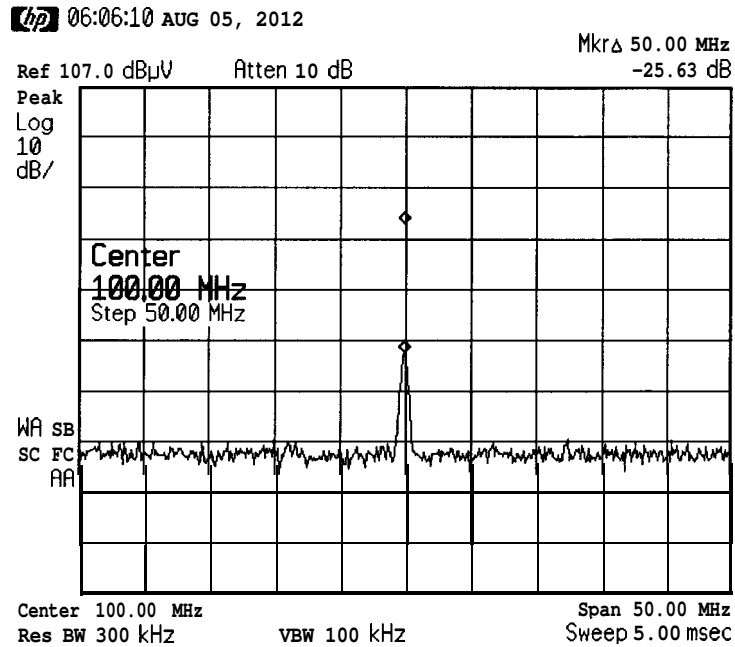
Figure 2-3 Frequency and Amplitude Difference Between Signals
