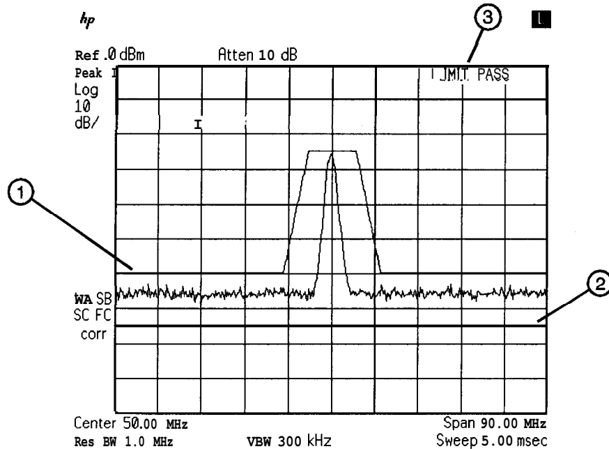
Figure 4-1 Typical Limit Line Display
