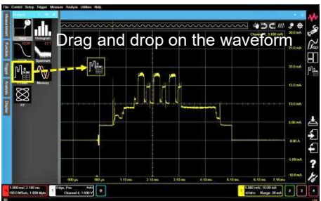
Figure 17. Automated power and current profiler results
